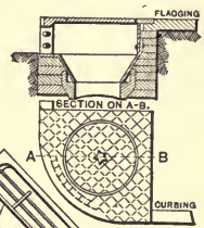
FIG. 5. STONE TOP INLET WITH CATCH-BASIN.
